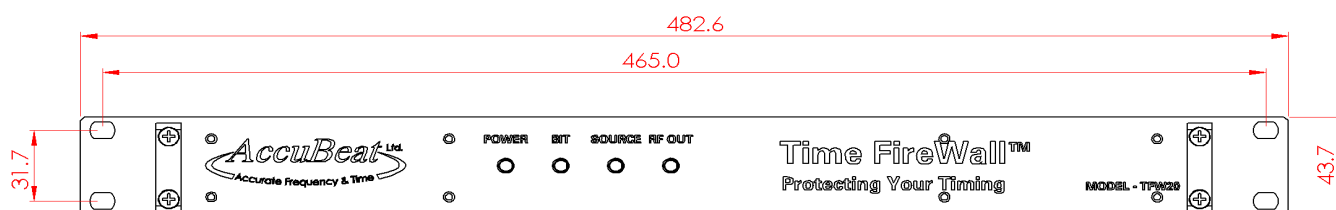
FRONT VIEW
