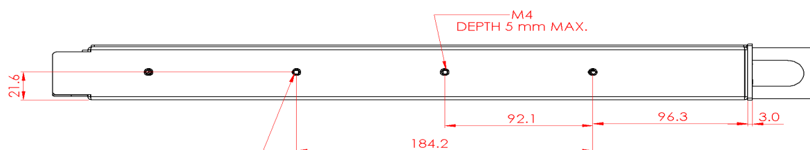
SIDE VIEW
